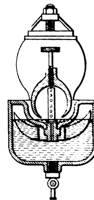
END VIEW.
